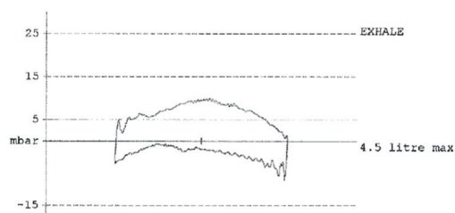
PRESSURE - VOLUME DIAGRAM AT DEPTH OF : 50,7 msw (166,4 fsw)
